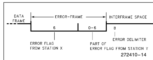
Figure 1. Error Frame Format
