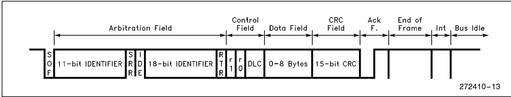
CAN Message Formats
